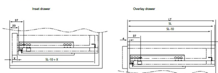
Installation dimensions
